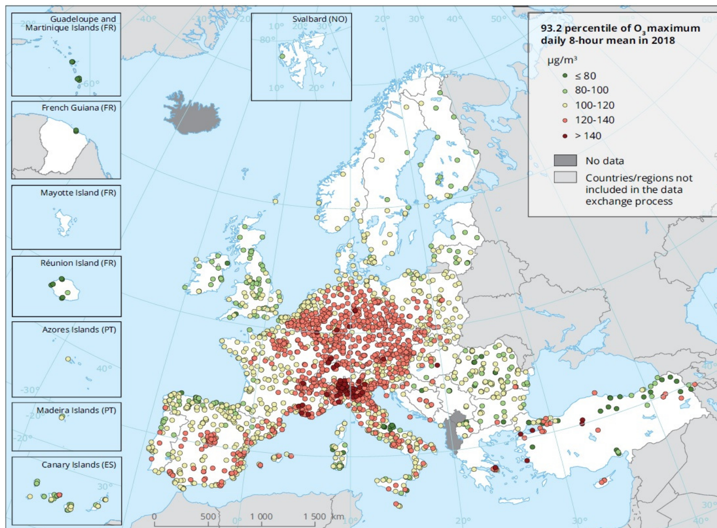
Map 5.1 Concentrations of O 3 in 2018
