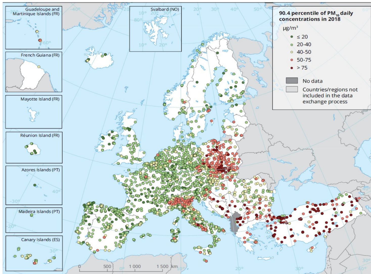
Map 4.1 Concentrations of PM 10 , 2018 — daily limit value
