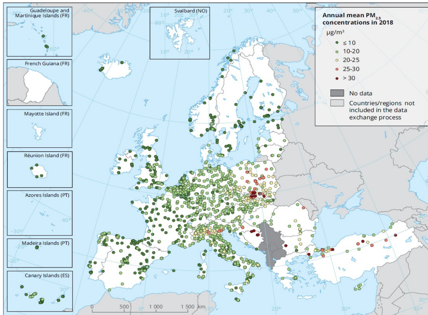
Map 4.3 Concentrations of PM 2.5 , 2018 — annual limit value
