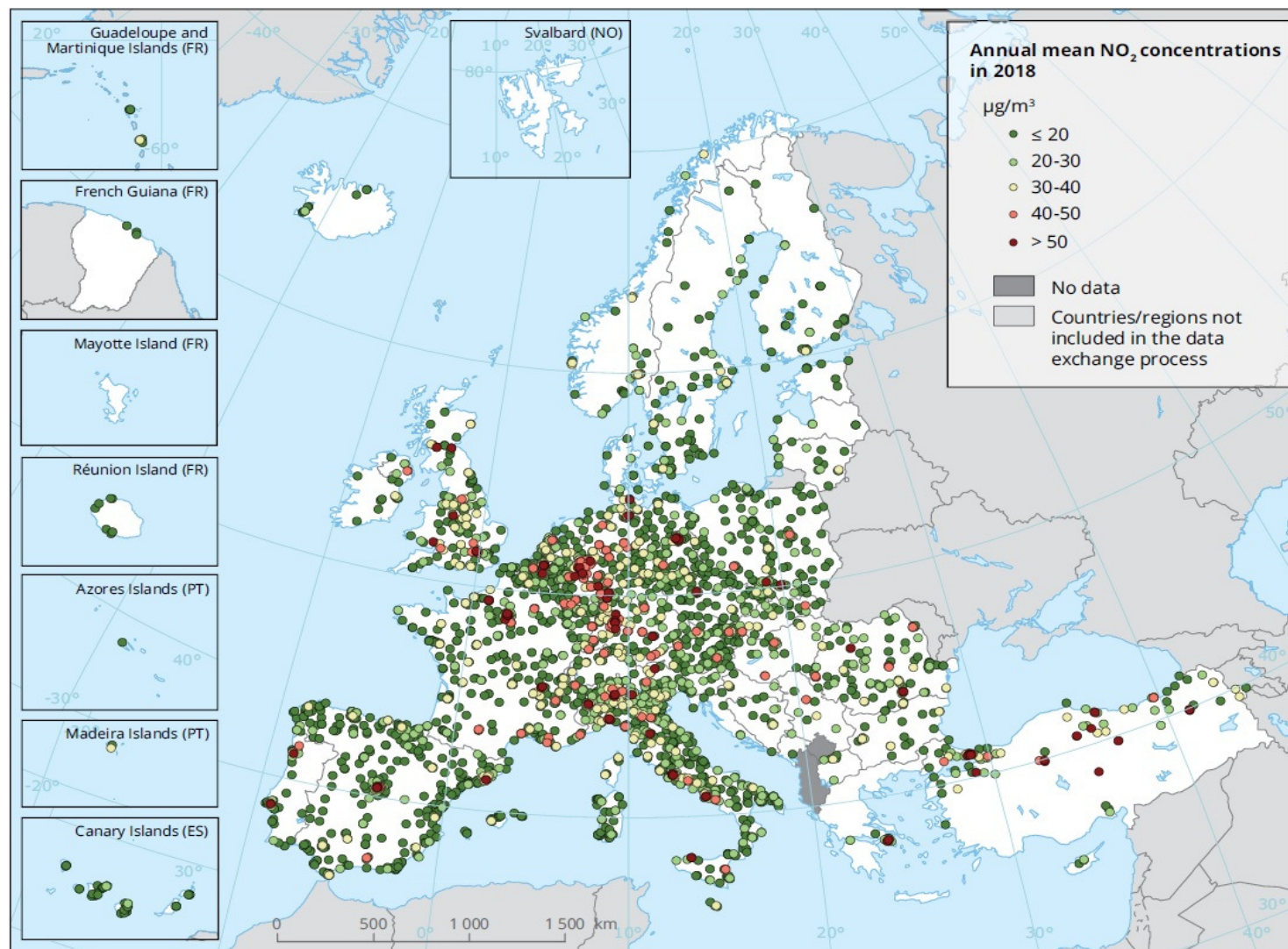
Map 6.1 Concentrations of NO 2 , 2018
