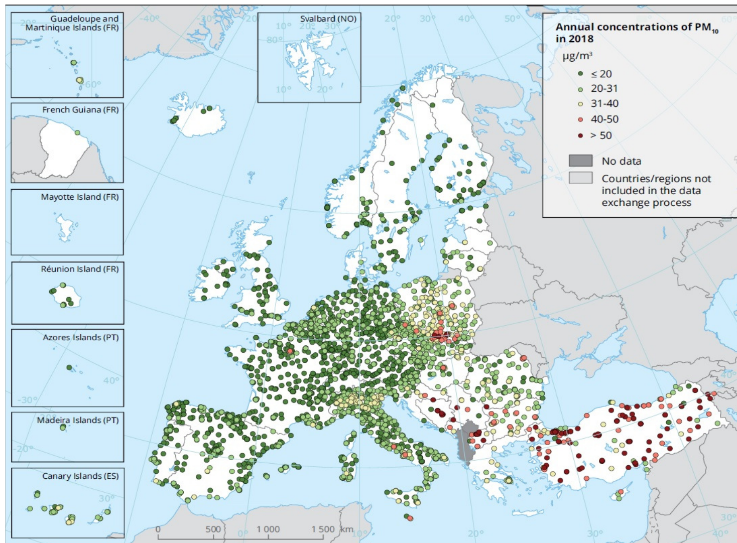
Map 4.2 Concentrations of PM 10 , 2018 — annual limit value
